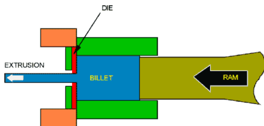
Figure 1: Direct extrusion process
