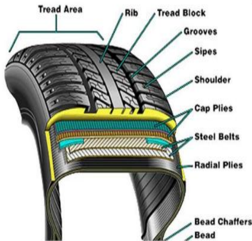
Passenger Car Tyre Cross Section
